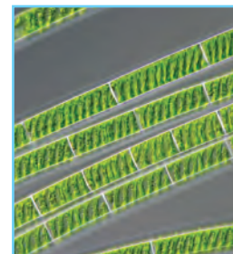
Spirogyra
