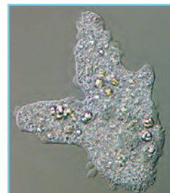
Amoeba
